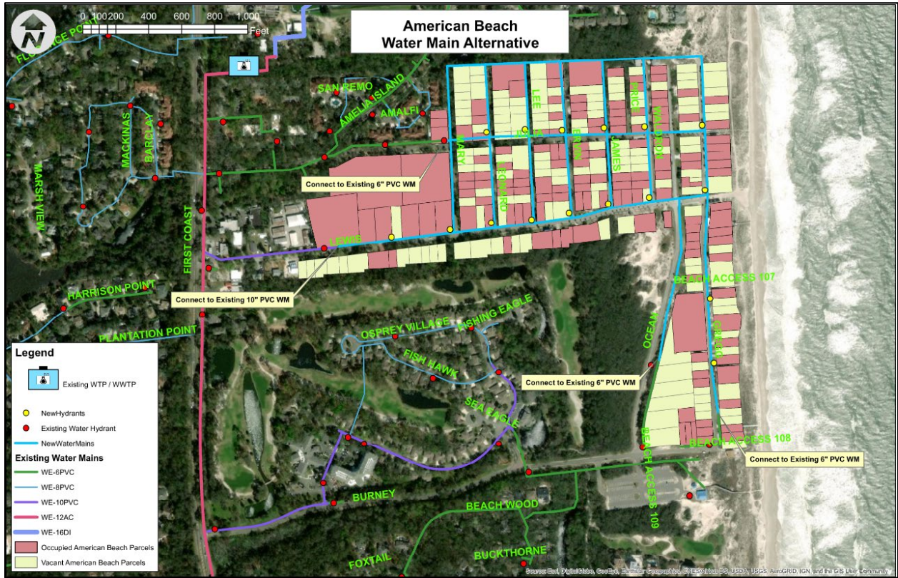
FIGURE 2: CENTRALIZED WATER PROJECT SITE PLAN
